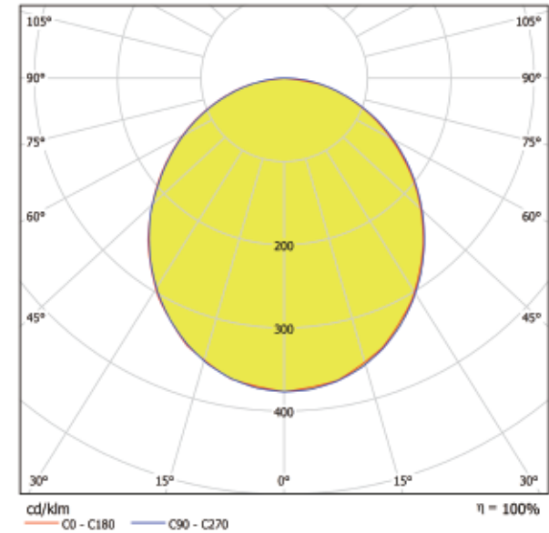
Photometric information corresponding at 24W 4000K.
